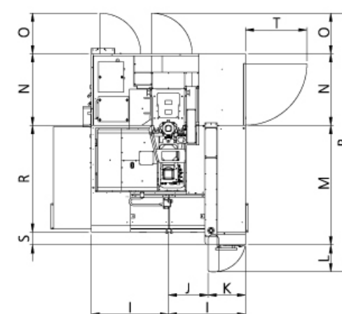
MACHINE DIMENSIONS
