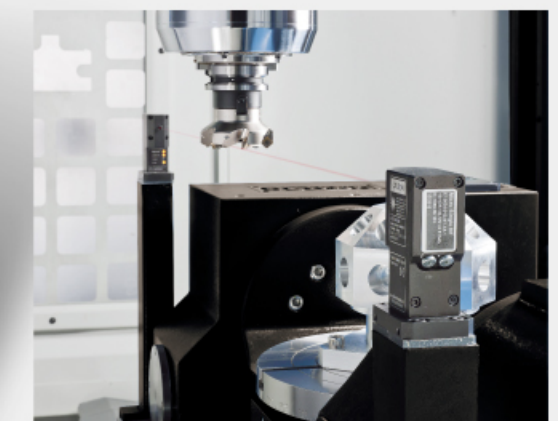
AUTOMATIC TOOL LENGTH MEASURING DEVICE (RENISHAW or BLUM)
